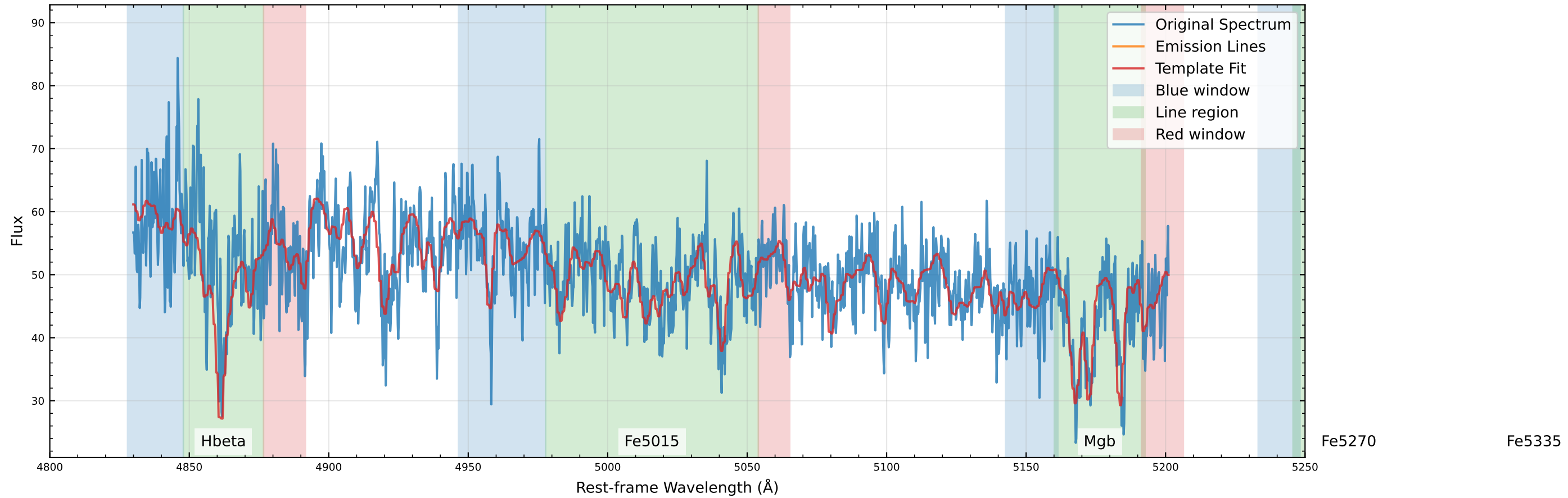
Original Data Comparison (v_star=37.8 km/s, v_gas=-11.4 km/s)
