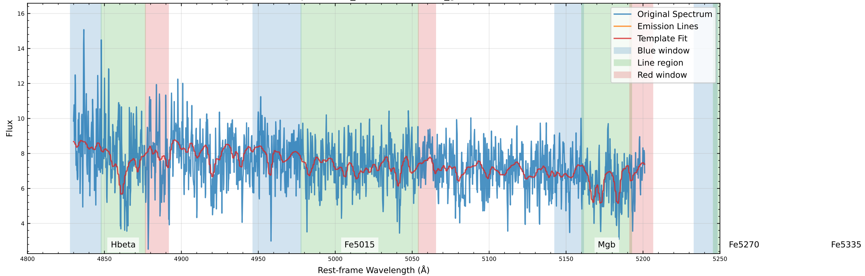
Original Data Comparison (v_star=44.3 km/s, v_gas=-117.9 km/s)
