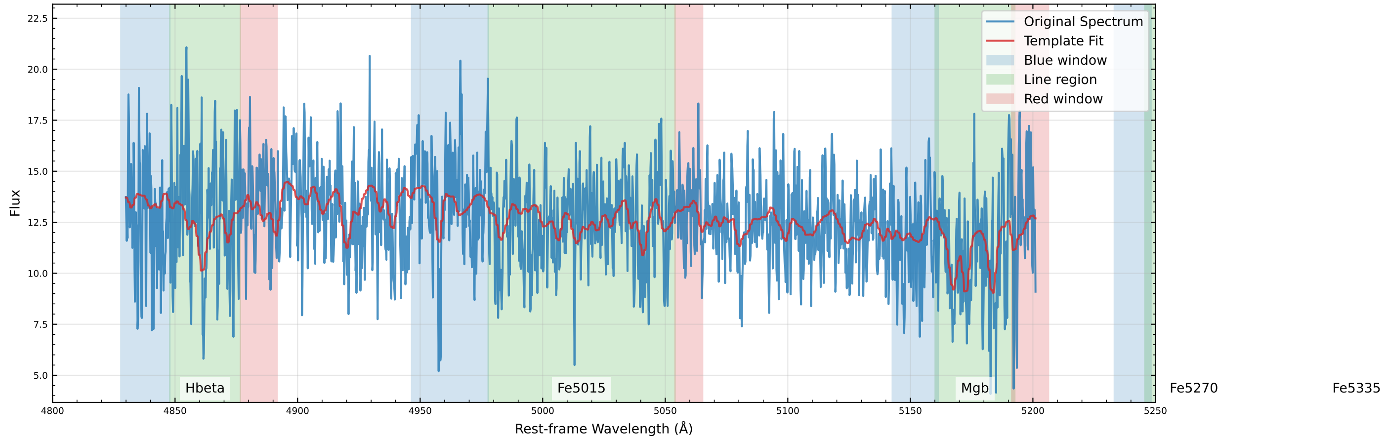
Original Data Comparison (v_star=32.7 km/s)
