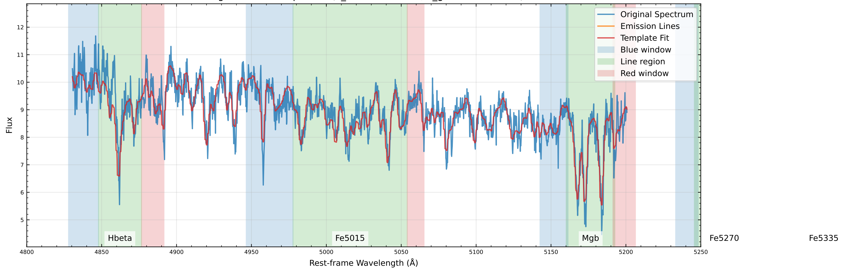
Original Data Comparison (v_star=20.4 km/s, v_gas=-279.6 km/s)
