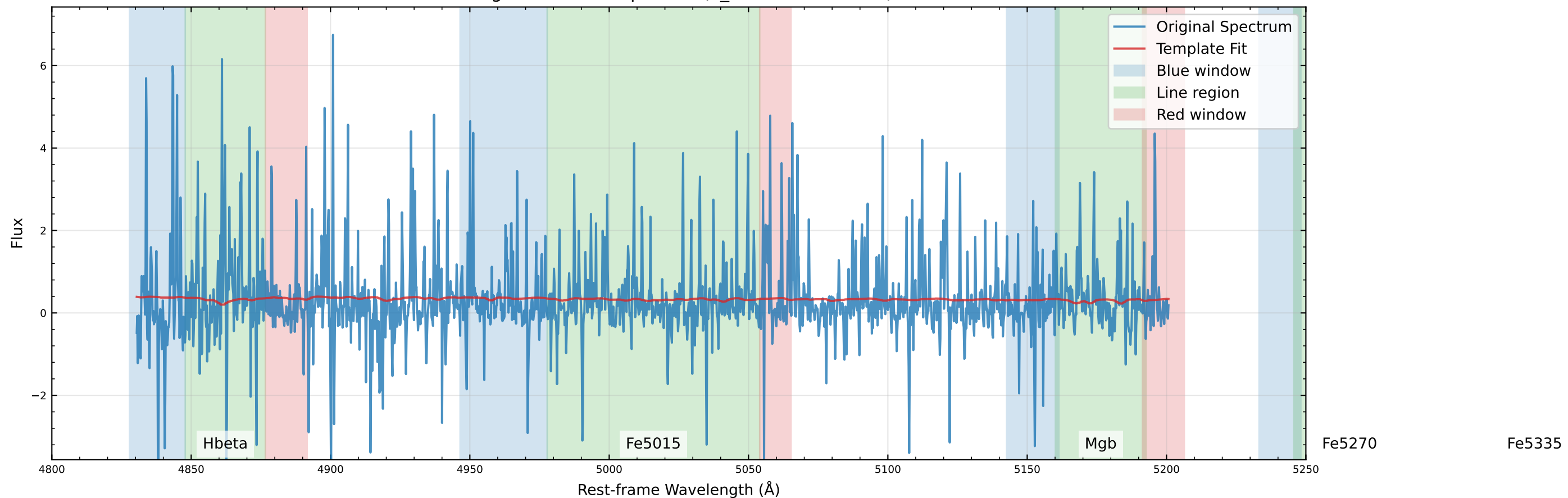
Original Data Comparison (v_star=-221.8 km/s)
