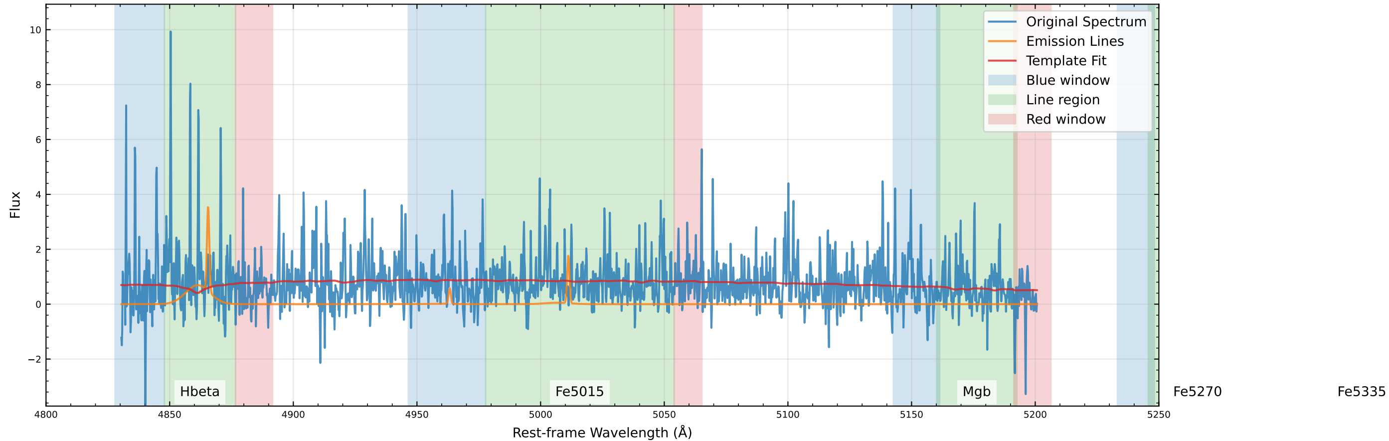
Original Data Comparison (v_star=-149.8 km/s, v_gas=-449.8 km/s)
