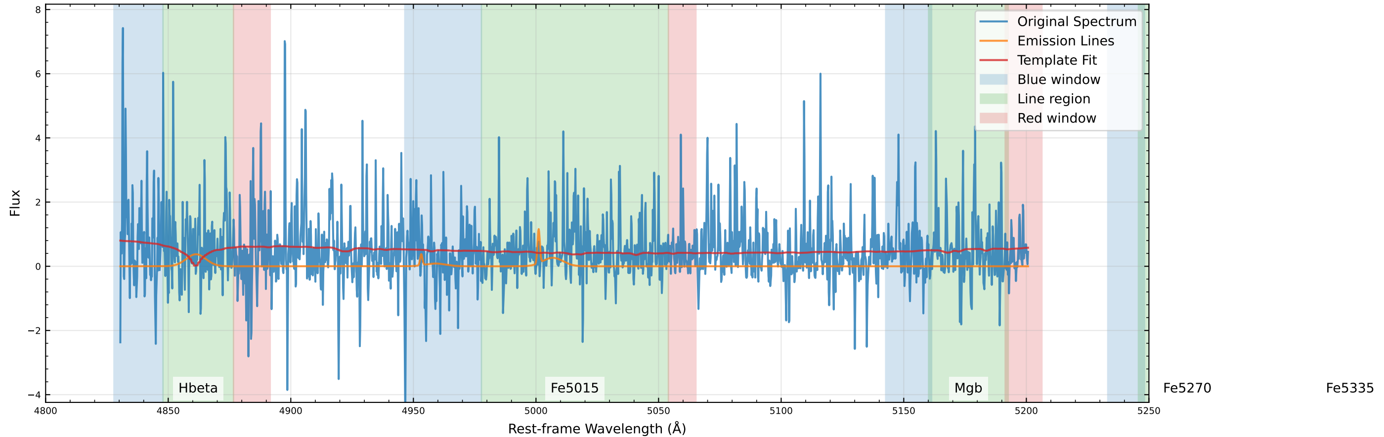
Original Data Comparison (v_star=-52.9 km/s, v_gas=247.1 km/s)
