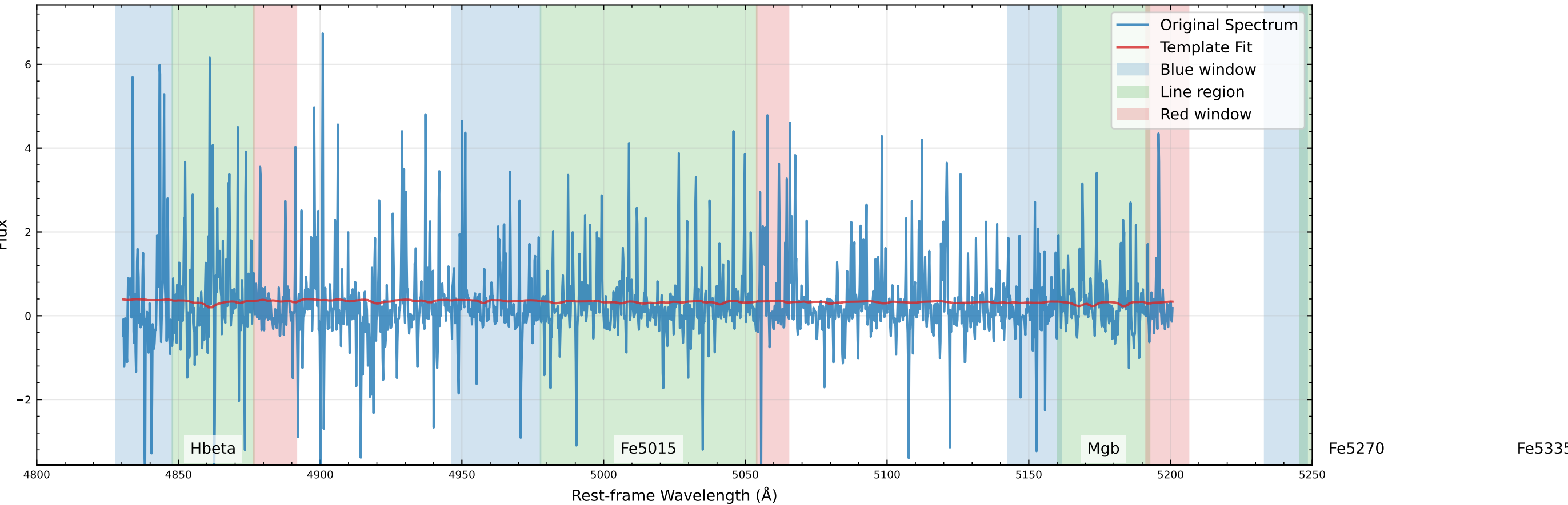
Original Data Comparison (v_star=-221.8 km/s)
