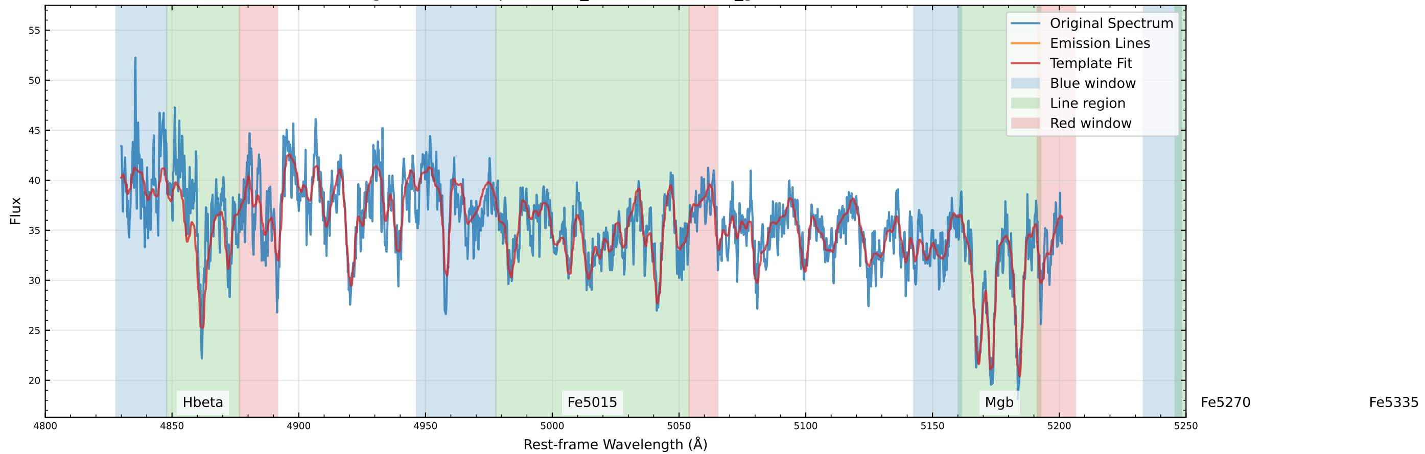
Original Data Comparison (v_star=33.5 km/s, v_gas=119.6 km/s)
