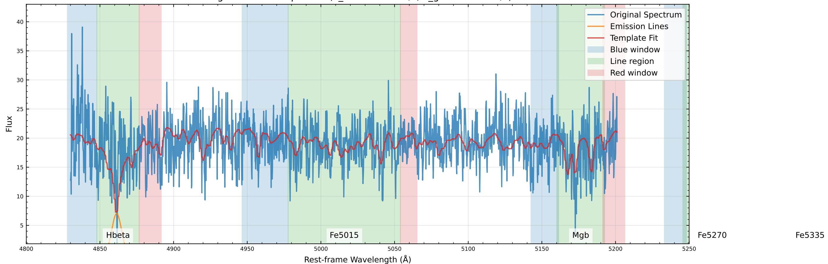
Original Data Comparison (v_star=29.8 km/s, v_gas=-29.8 km/s)
