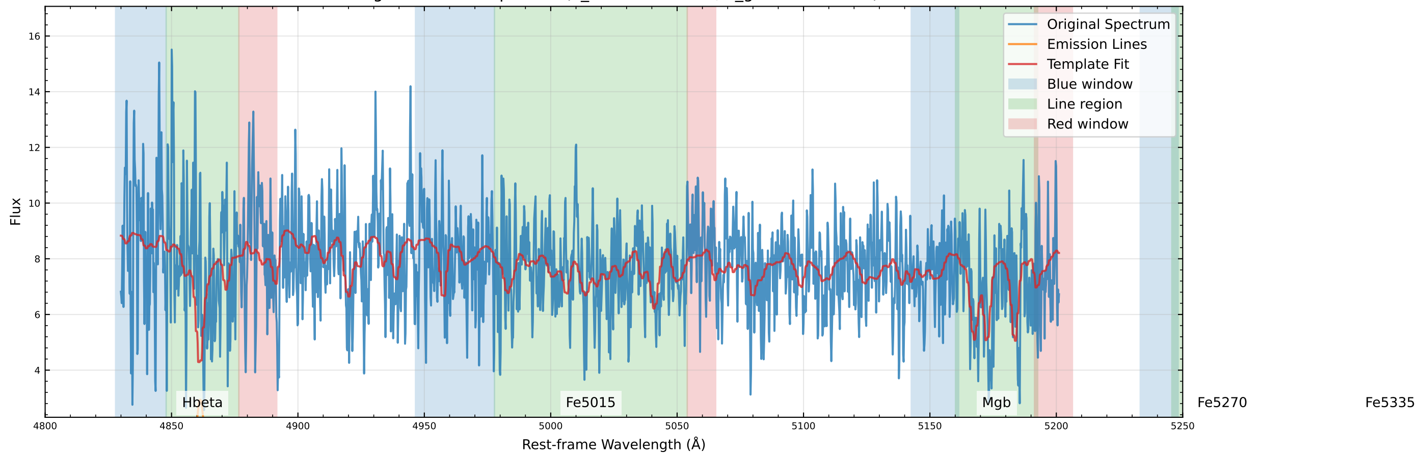
Original Data Comparison (v_star=58.3 km/s, v_gas=-70.6 km/s)
