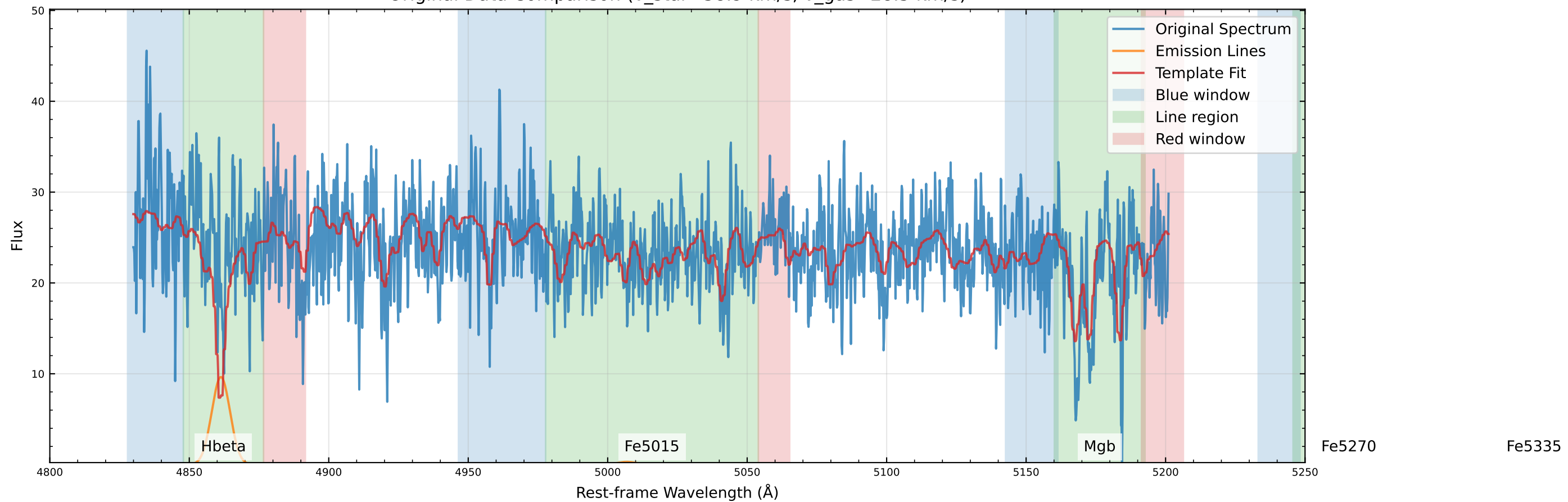
Original Data Comparison (v_star=38.9 km/s, v_gas=28.5 km/s)
