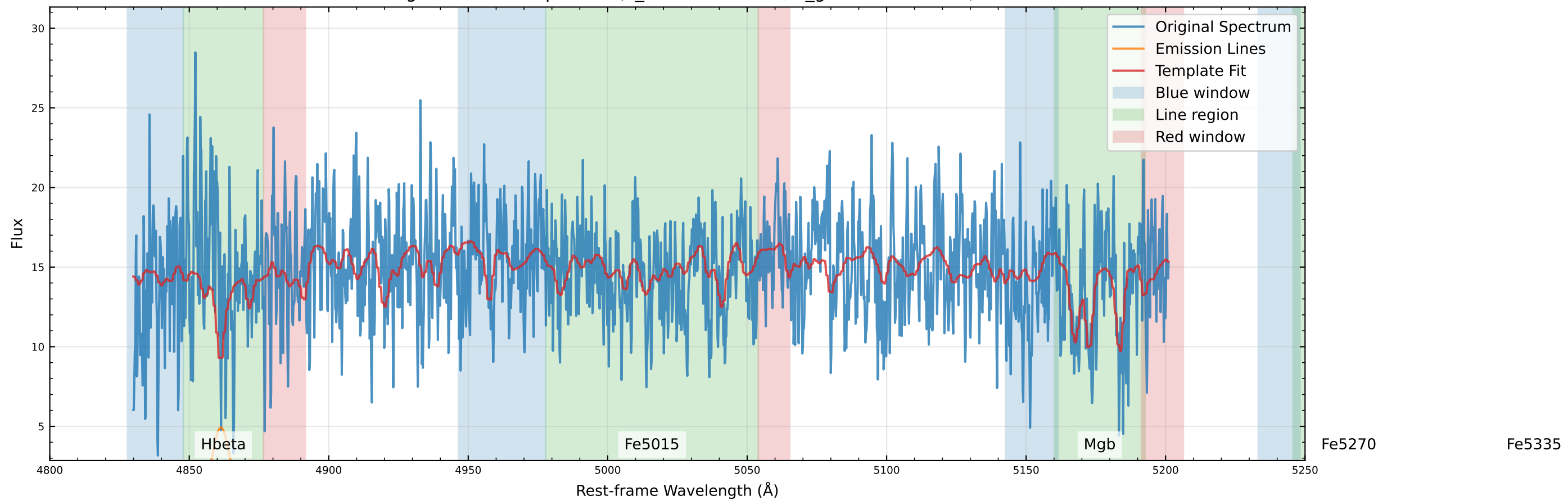
Original Data Comparison (v_star=43.6 km/s, v_gas=-214.2 km/s)
