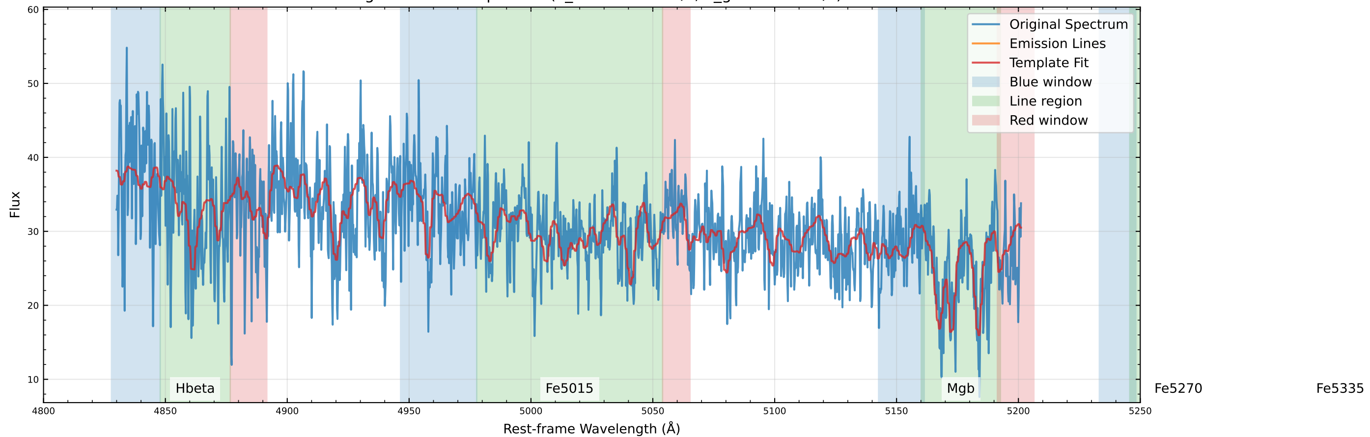
Original Data Comparison (v_star=33.2 km/s, v_gas=-2.1 km/s)
