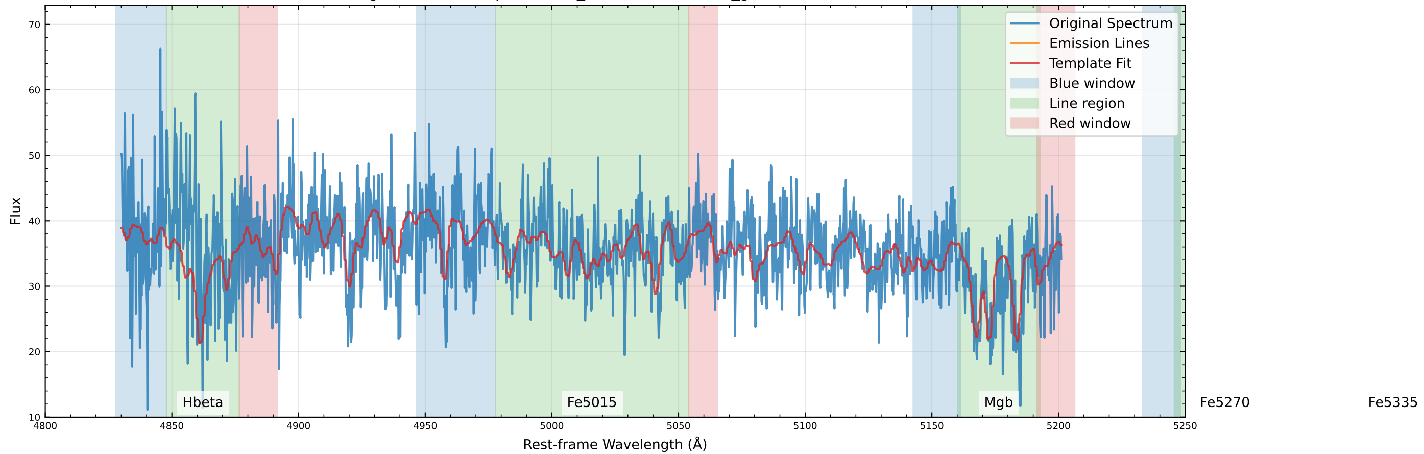
Original Data Comparison (v_star=42.1 km/s, v_gas=-250.5 km/s)
