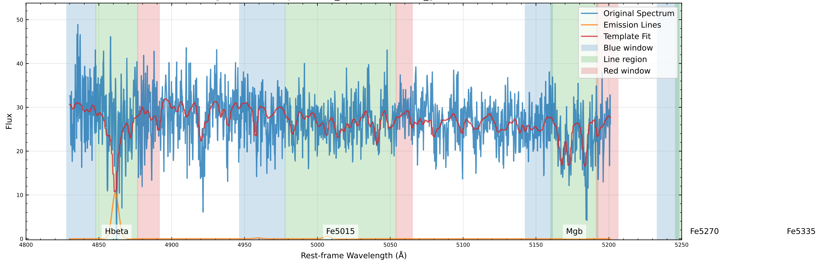
Original Data Comparison (v_star=45.6 km/s, v_gas=-52.0 km/s)
