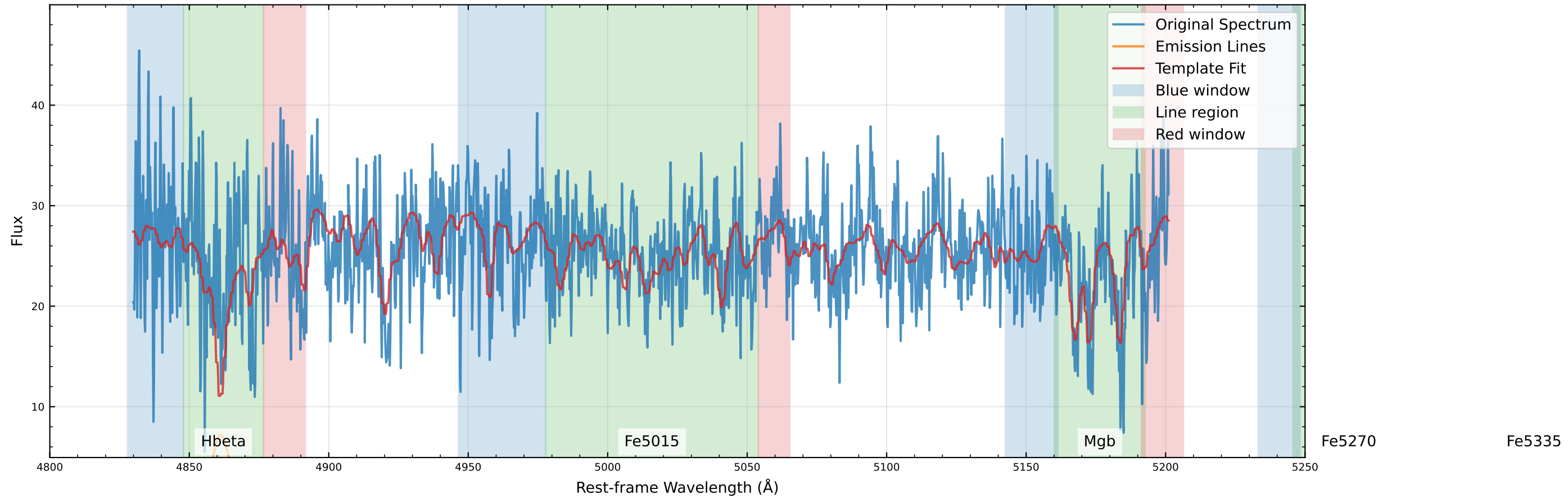
Original Data Comparison (v_star=35.5 km/s, v_gas=101.6 km/s)
