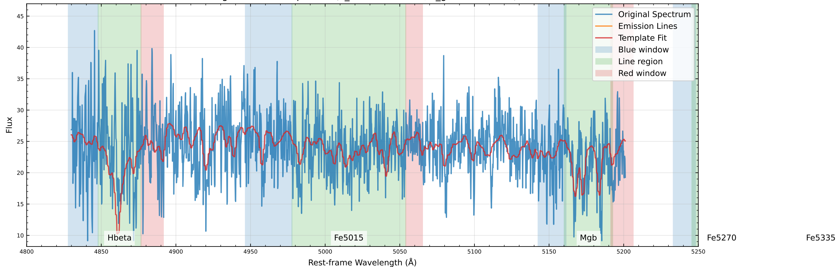
Original Data Comparison (v_star=41.4 km/s, v_gas=16.9 km/s)
