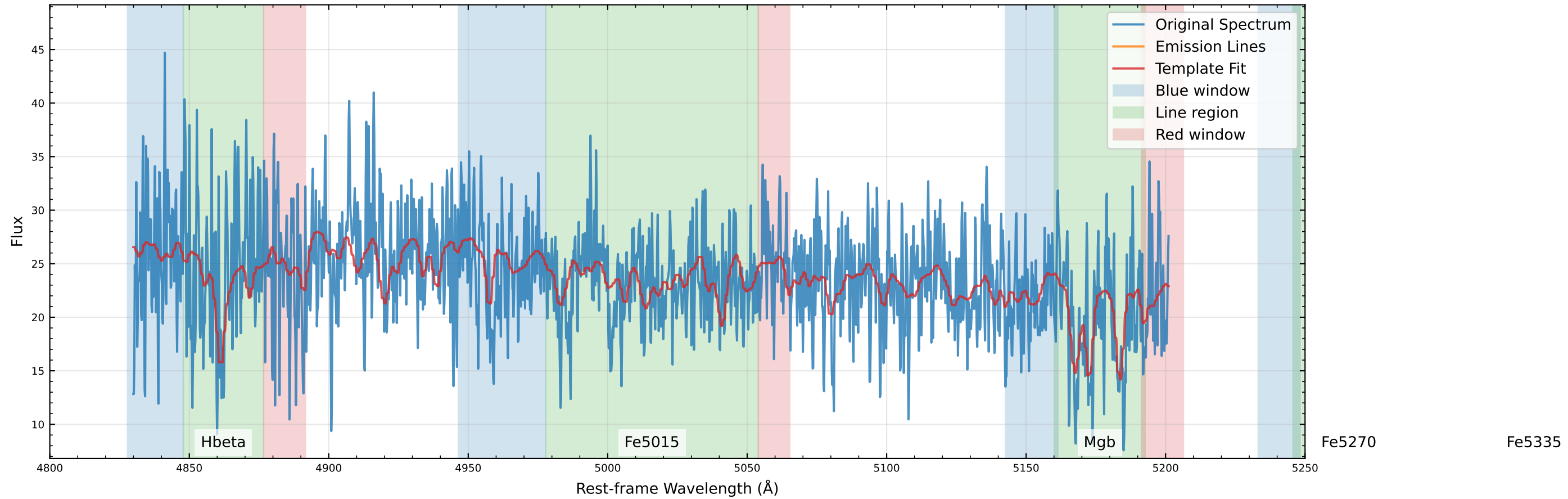
Original Data Comparison ( v_{\text{star}}=32.6 km/s, v_{\text{gas}}=332.6 km/s)
