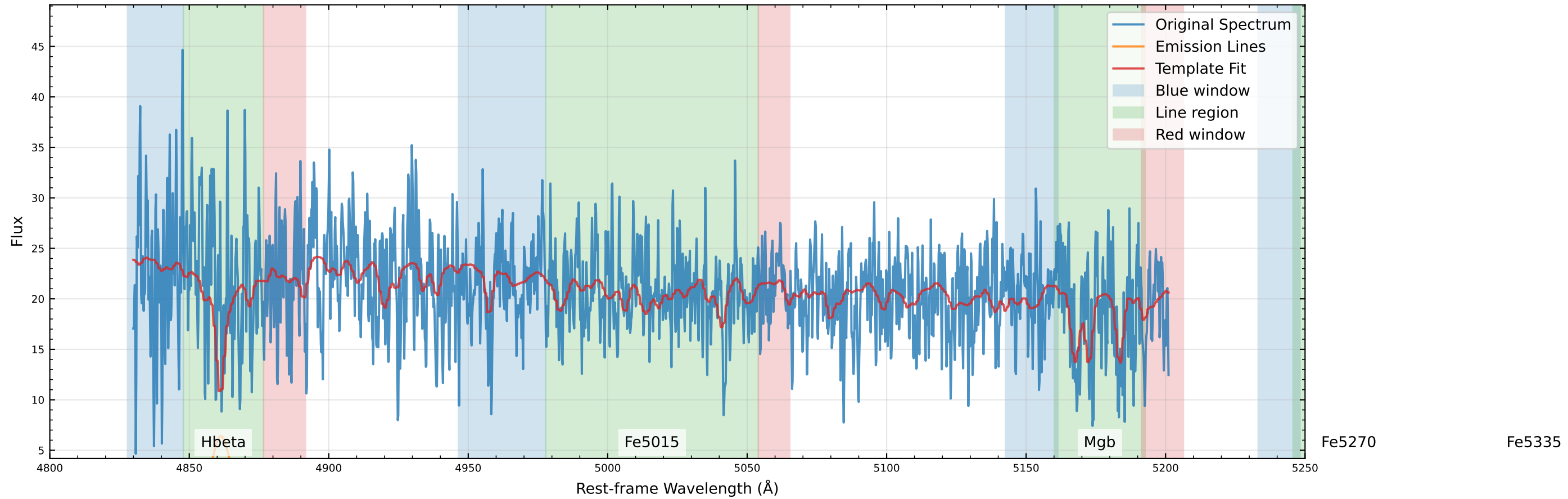
Original Data Comparison (v_star=28.9 km/s, v_gas=-72.6 km/s)
