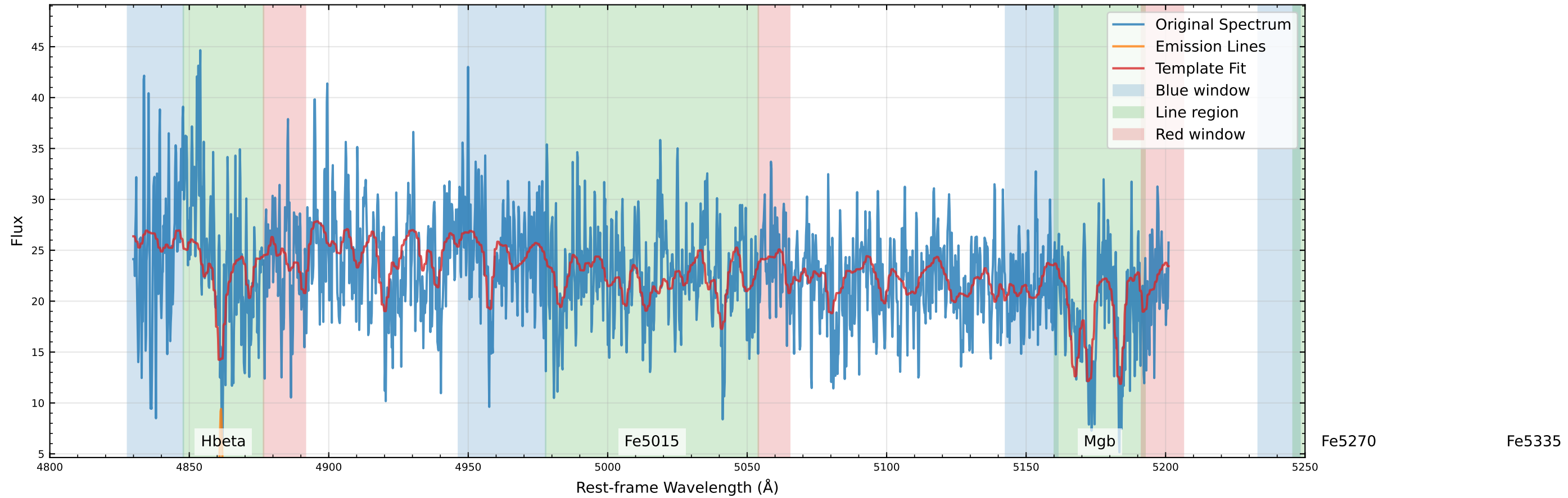
Original Data Comparison (v_star=48.2 km/s, v_gas=146.7 km/s)
