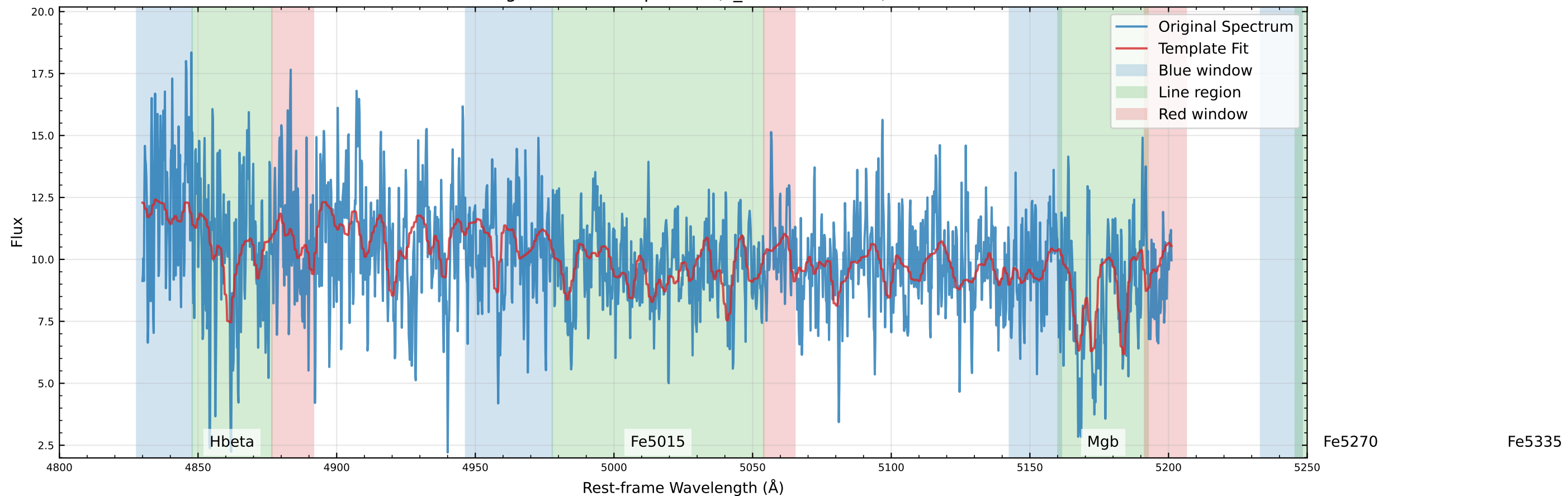
Original Data Comparison (v_star=61.0 km/s)
