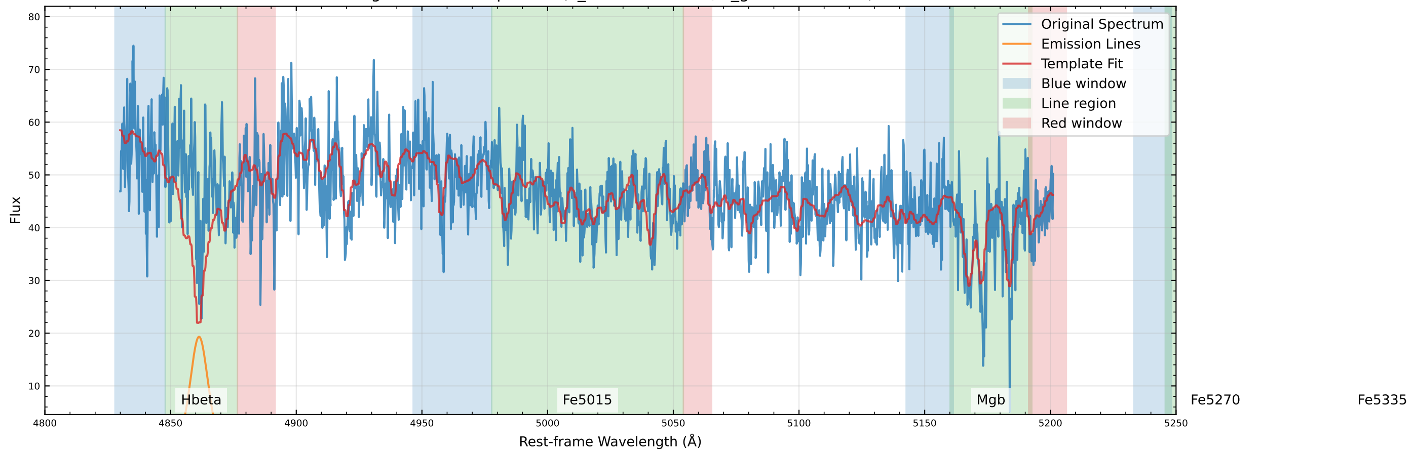
Original Data Comparison (v_star=25.3 km/s, v_gas=-48.1 km/s)
