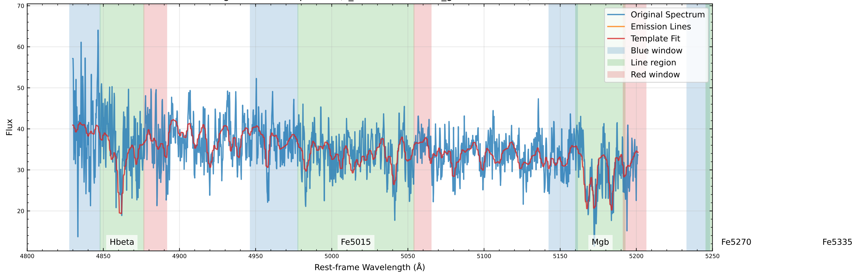
Original Data Comparison ( v_{\text{star}}=31.5 km/s, v_{\text{gas}}=103.4 km/s)
