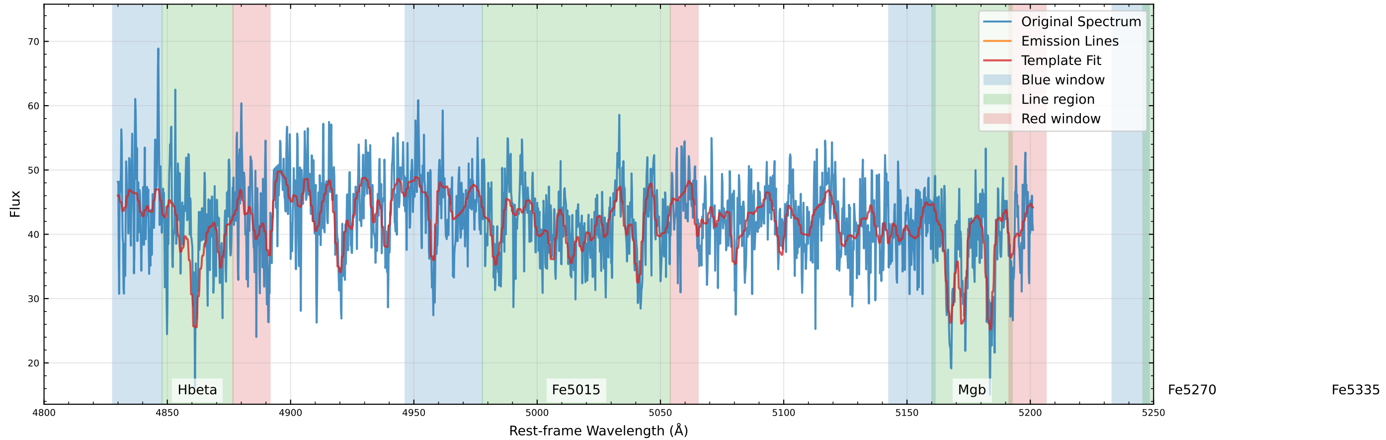
Original Data Comparison (v_star=27.1 km/s, v_gas=-75.2 km/s)
