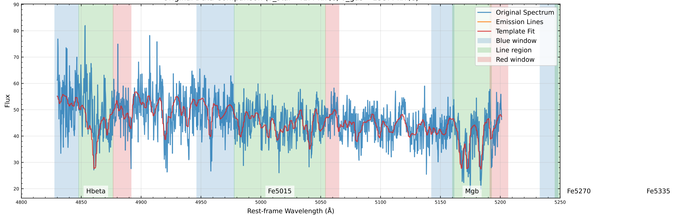
Original Data Comparison (v_star=41.4 km/s, v_gas=-153.4 km/s)
