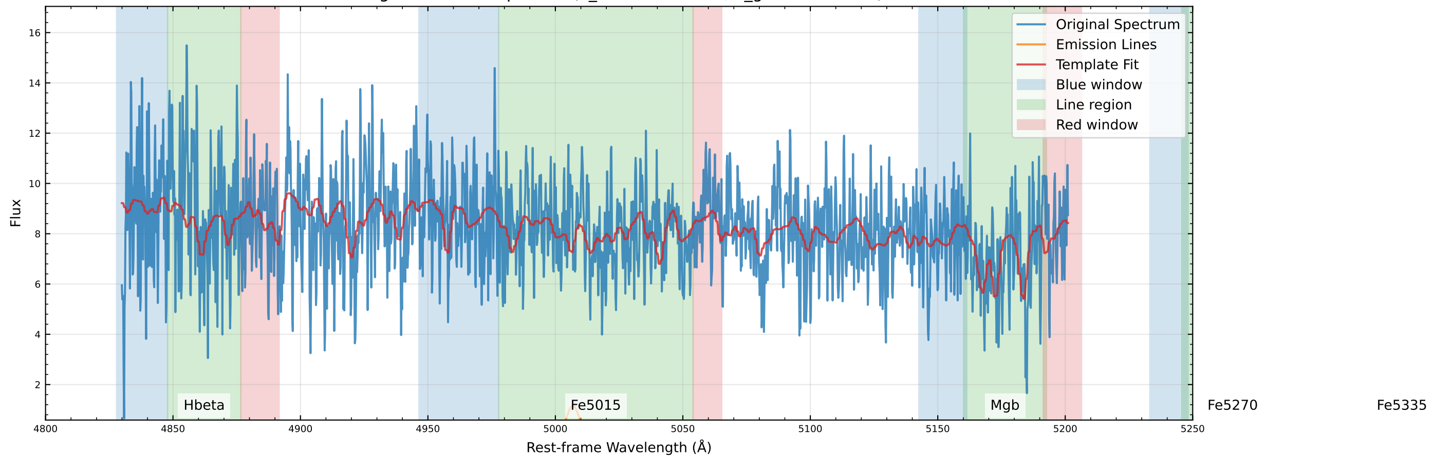
Original Data Comparison (v_star=59.0 km/s, v_gas=30.1 km/s)
