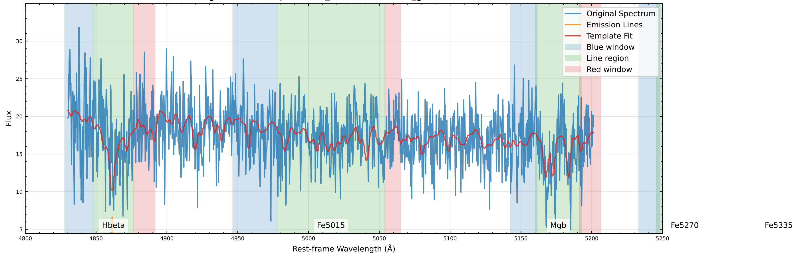
Original Data Comparison (v_star=51.5 km/s, v_gas=-24.0 km/s)
