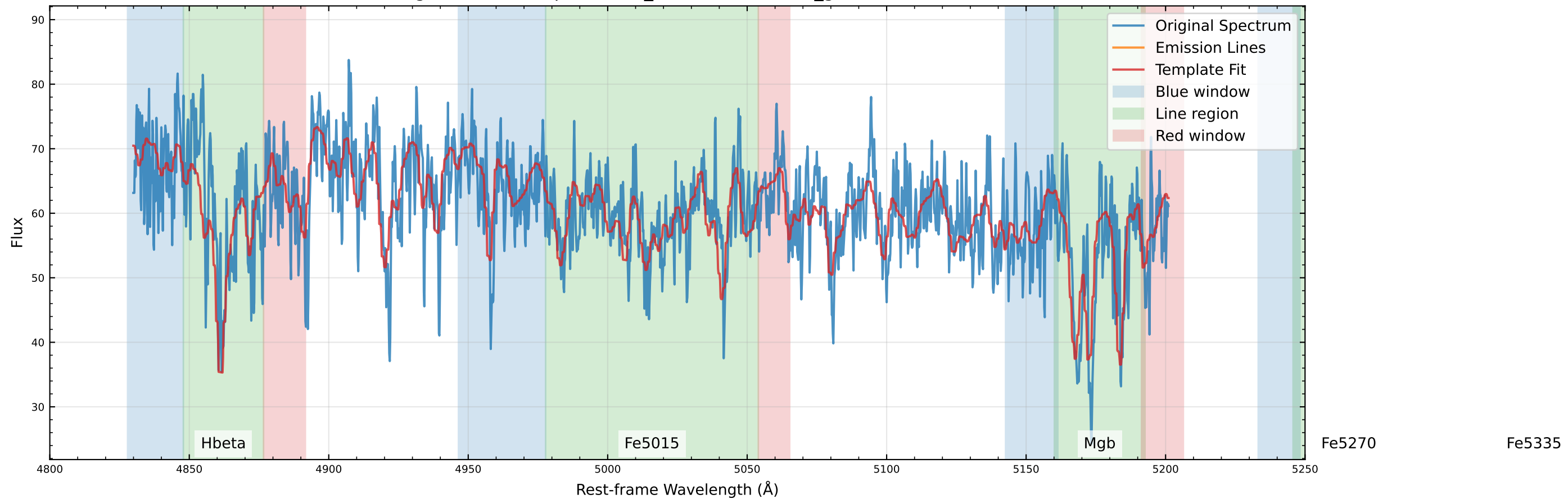
Original Data Comparison (v_star=51.1 km/s, v_gas=88.6 km/s)
