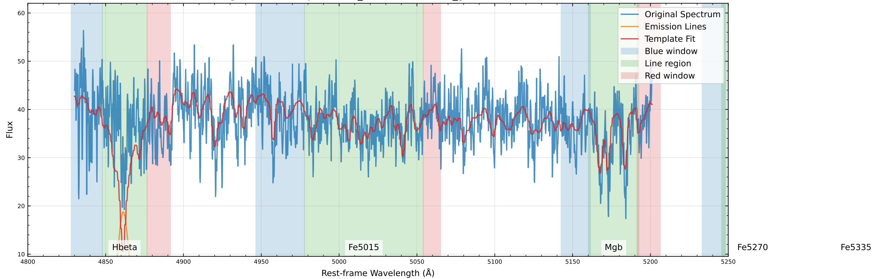
Original Data Comparison (v_star=31.6 km/s, v_gas=-33.0 km/s)
