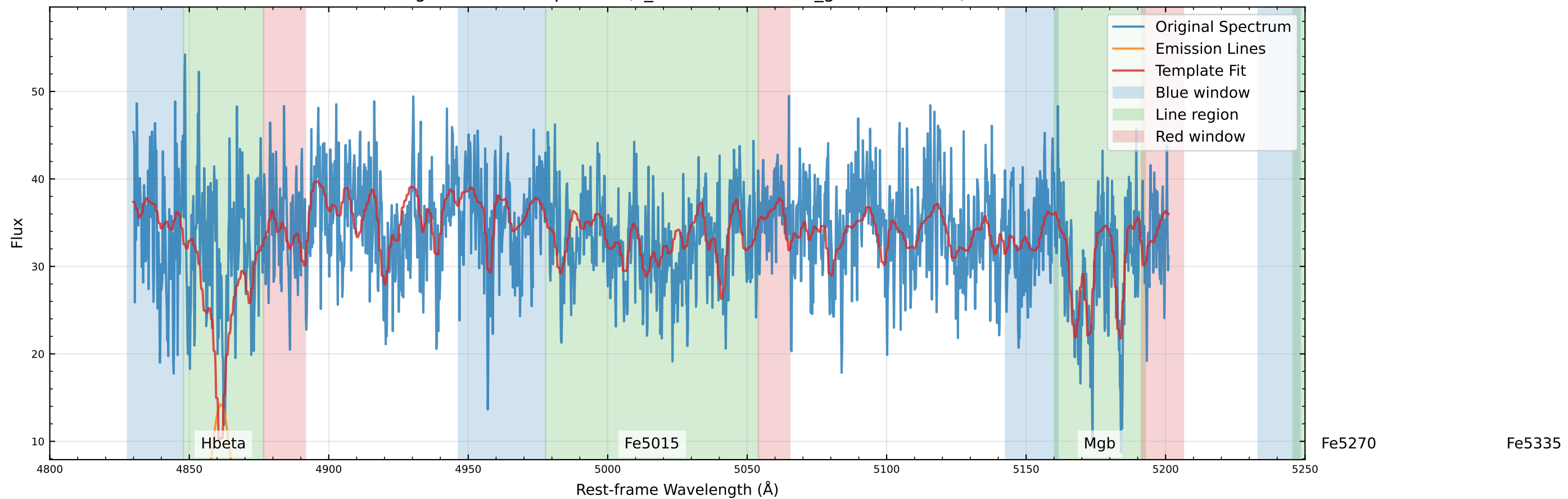
Original Data Comparison (v_star=41.4 km/s, v_gas=10.4 km/s)
