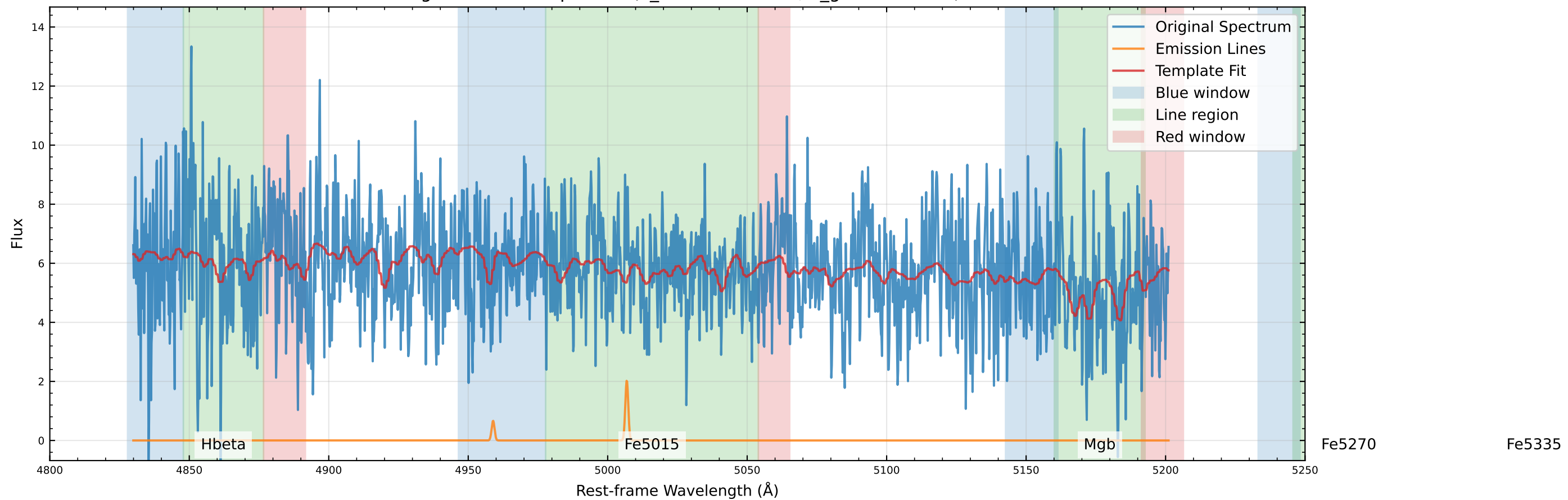
Original Data Comparison (v_star=64.7 km/s, v_gas=2.8 km/s)
