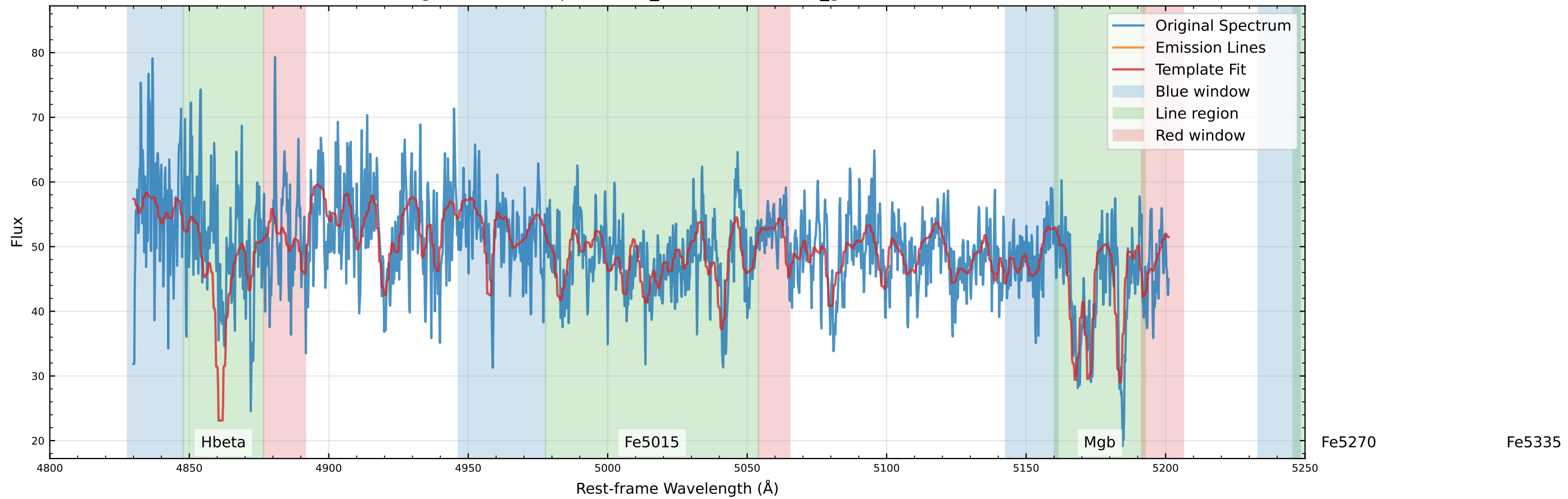
Original Data Comparison (v_star=49.8 km/s, v_gas=1.9 km/s)
