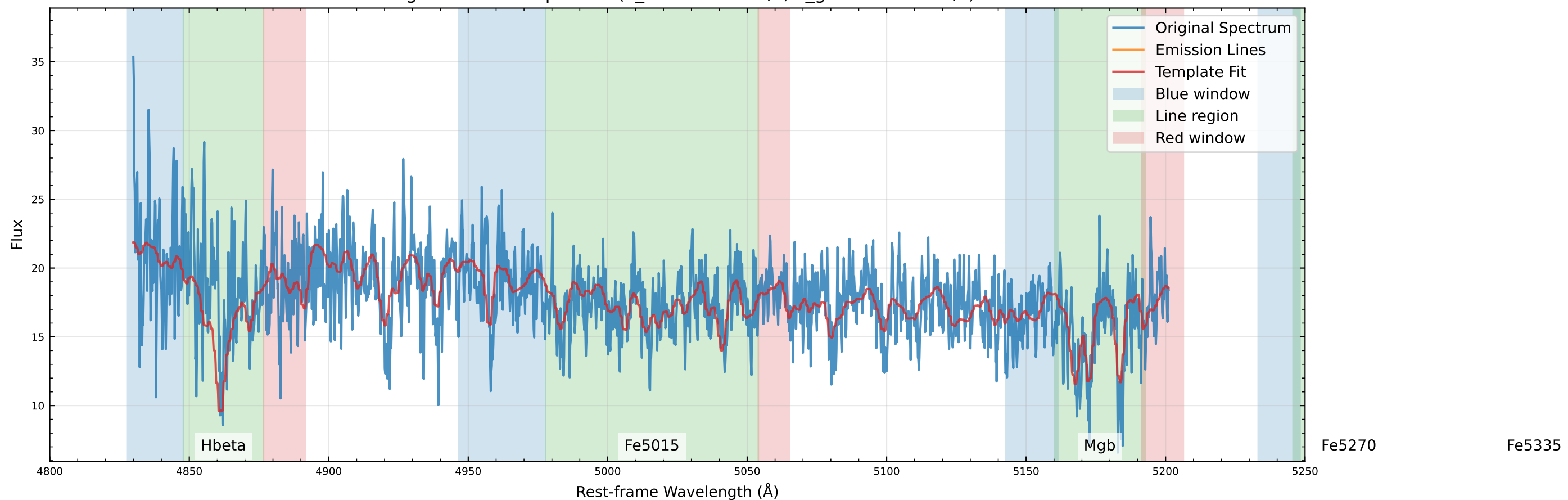
Original Data Comparison (v_star=18.5 km/s, v_gas=-104.3 km/s)
