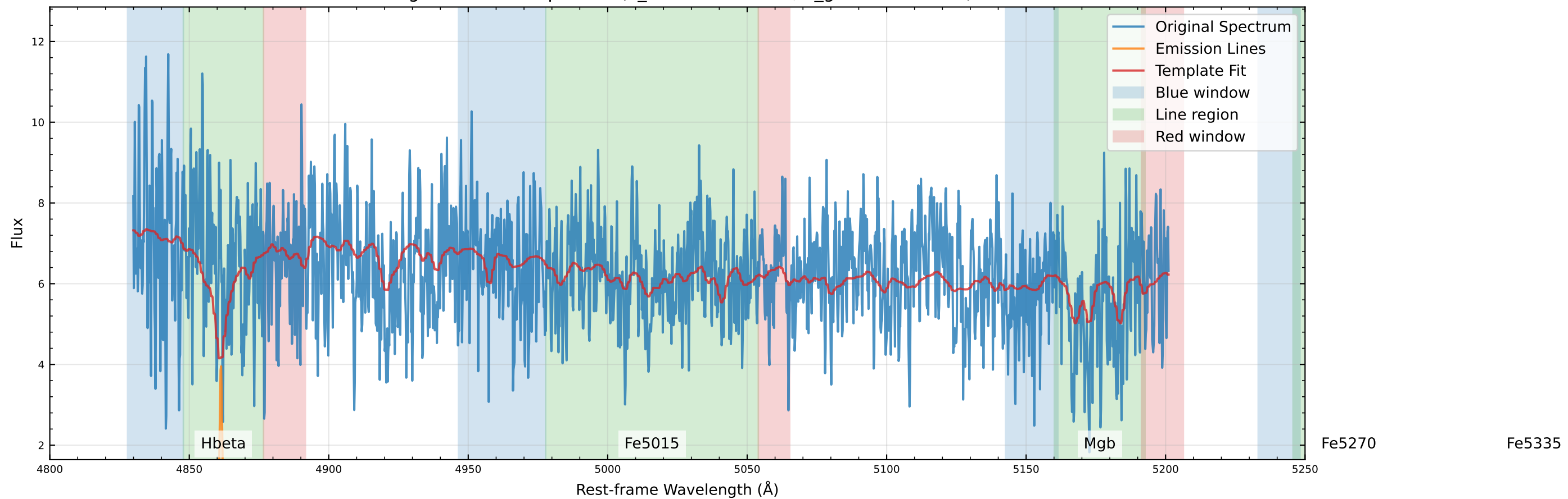
Original Data Comparison (v_star=-22.2 km/s, v_gas=-22.2 km/s)
