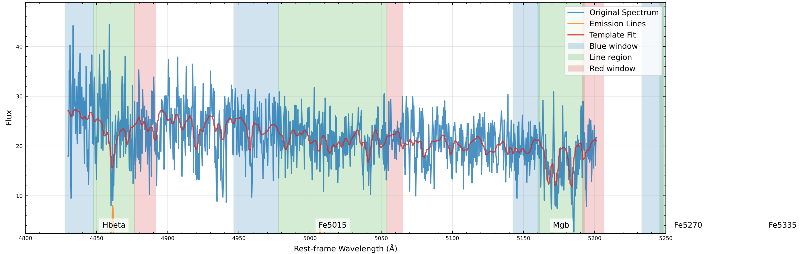
Original Data Comparison ( v_{\text{star}}=79.0 km/s, v_{\text{gas}}=104.2 km/s)
