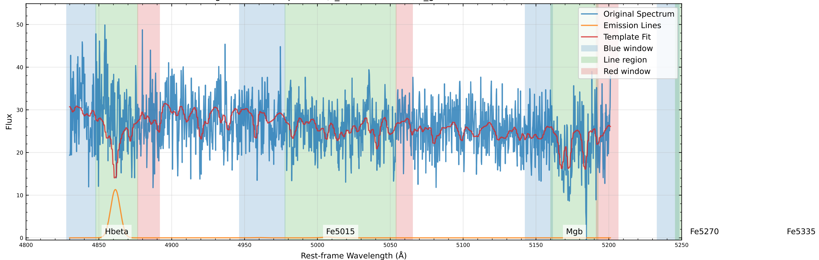
Original Data Comparison (v_star=63.6 km/s, v_gas=-23.7 km/s)
