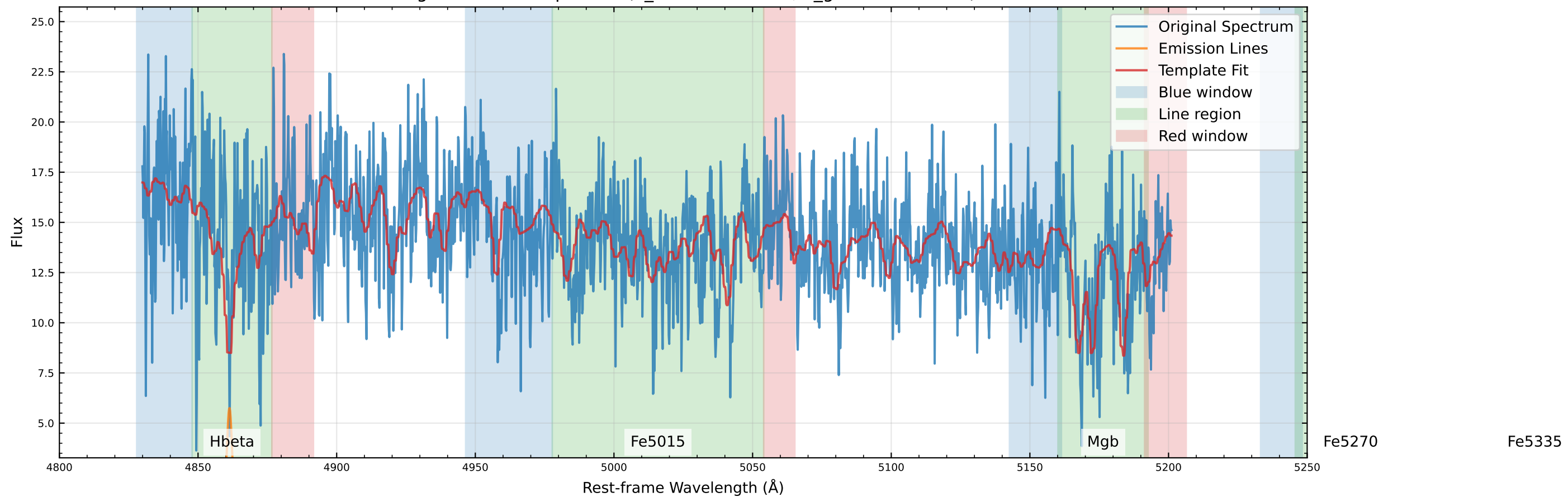
Original Data Comparison (v_star=78.7 km/s, v_gas=139.3 km/s)
