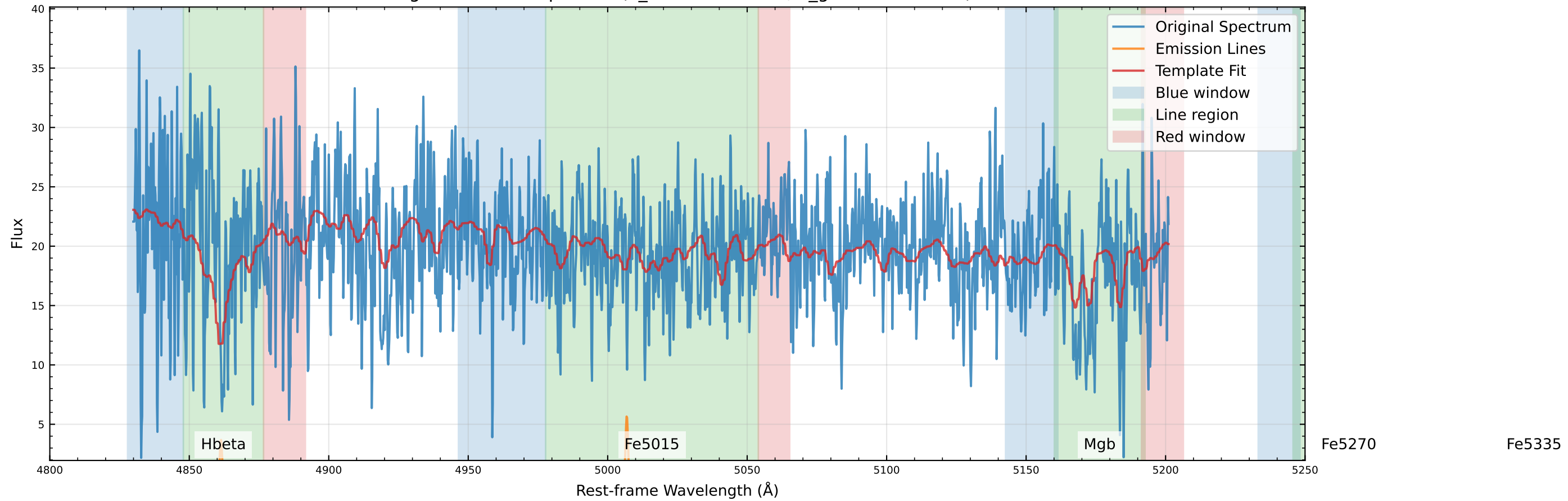
Original Data Comparison (v_star=55.7 km/s, v_gas=131.7 km/s)
