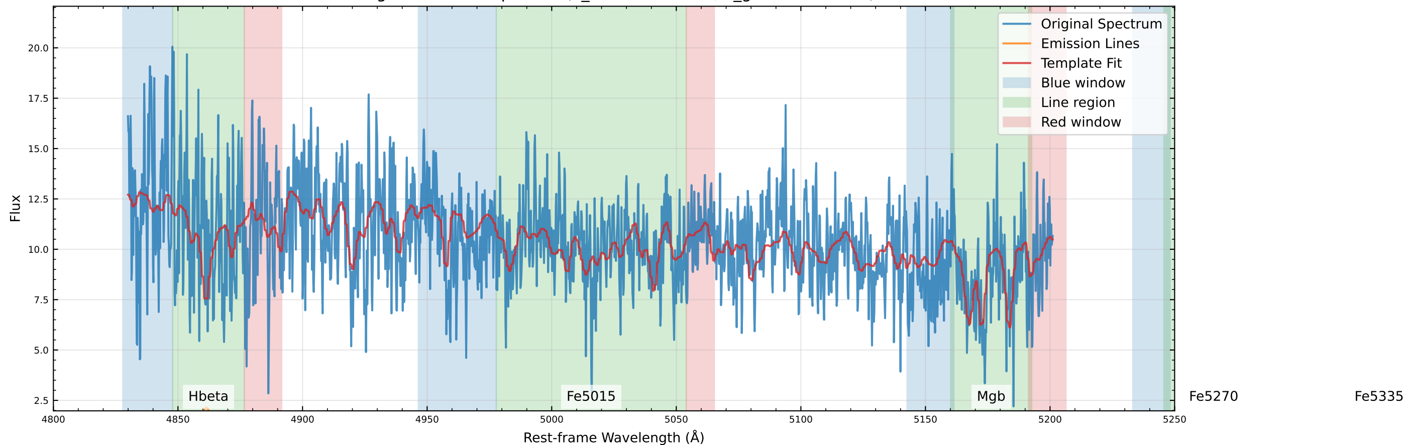
Original Data Comparison (v_star=39.6 km/s, v_gas=-57.9 km/s)
