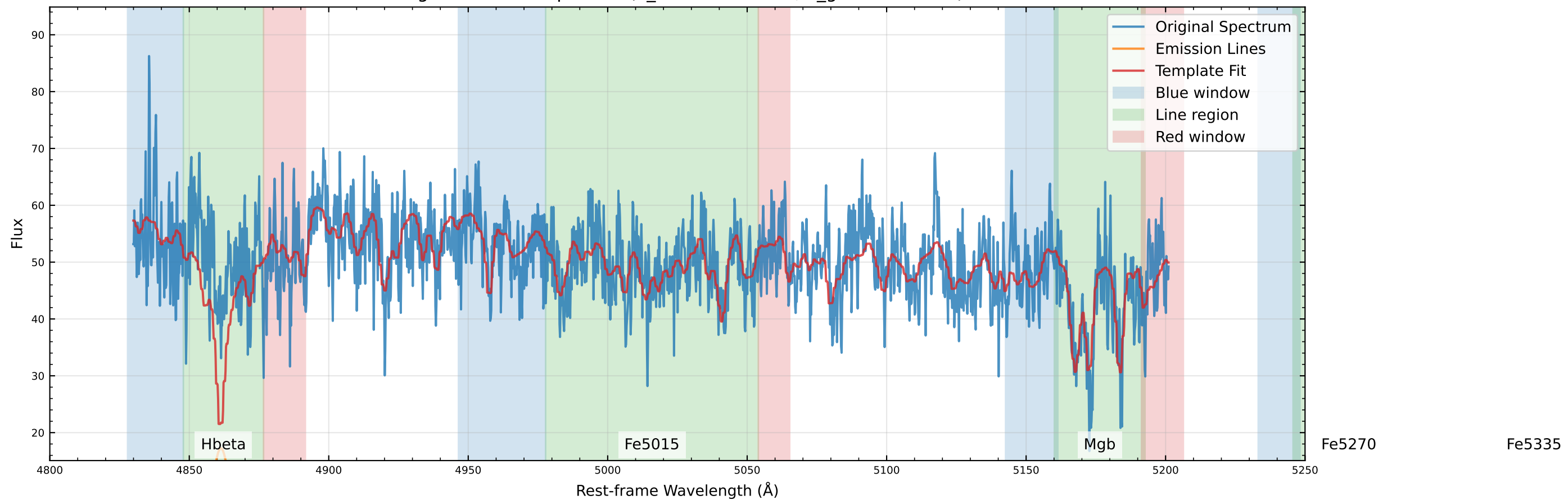
Original Data Comparison (v_star=22.9 km/s, v_gas=-2.7 km/s)
