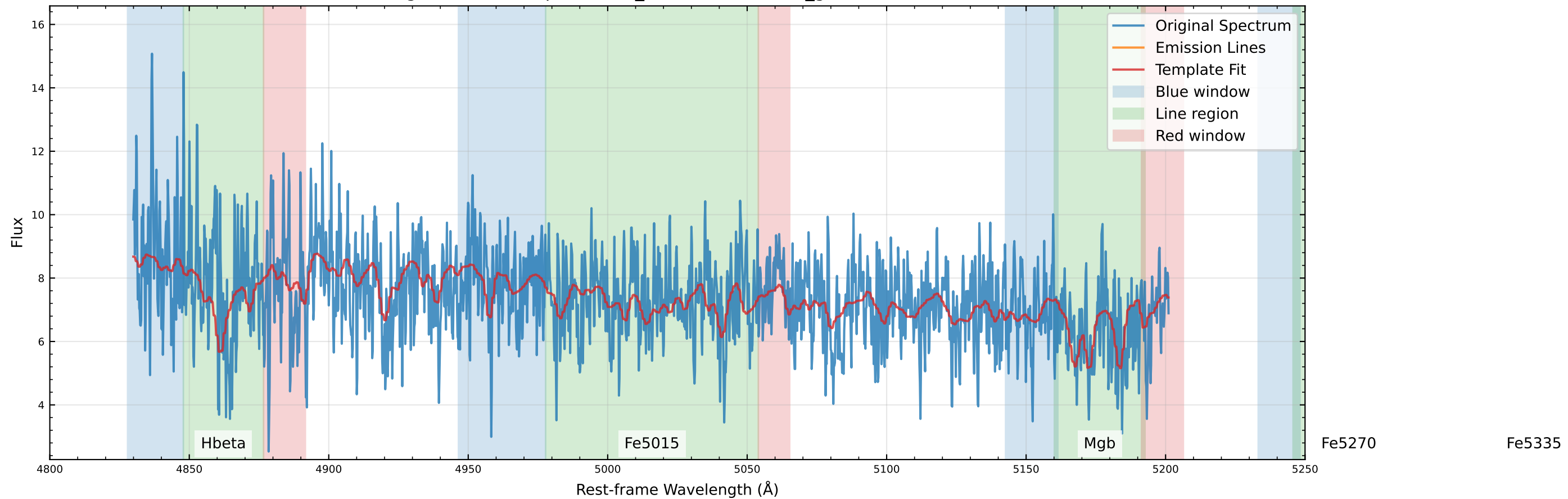
Original Data Comparison ( v_{\text{star}}=44.3 km/s, v_{\text{gas}}=-117.9 km/s)
