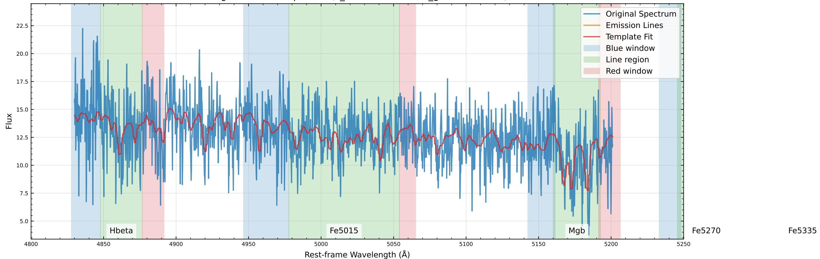
Original Data Comparison (v_star=31.6 km/s, v_gas=22.5 km/s)
