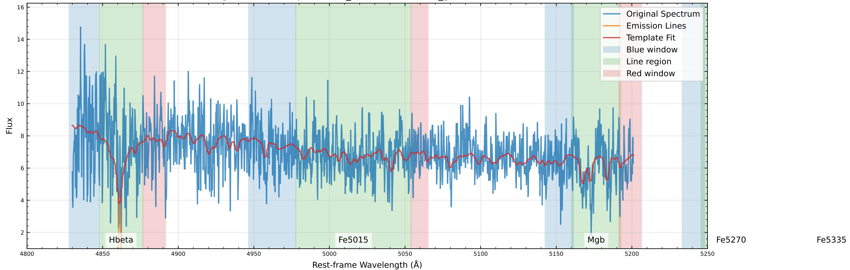
Original Data Comparison ( v_{\text{star}}=49.7 km/s, v_{\text{gas}}=141.9 km/s)
