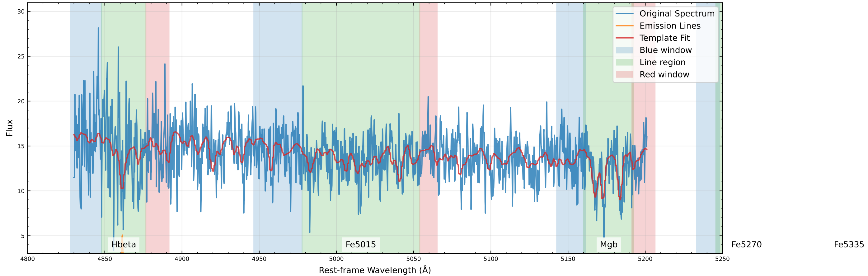
Original Data Comparison (v_star=69.0 km/s, v_gas=156.6 km/s)
