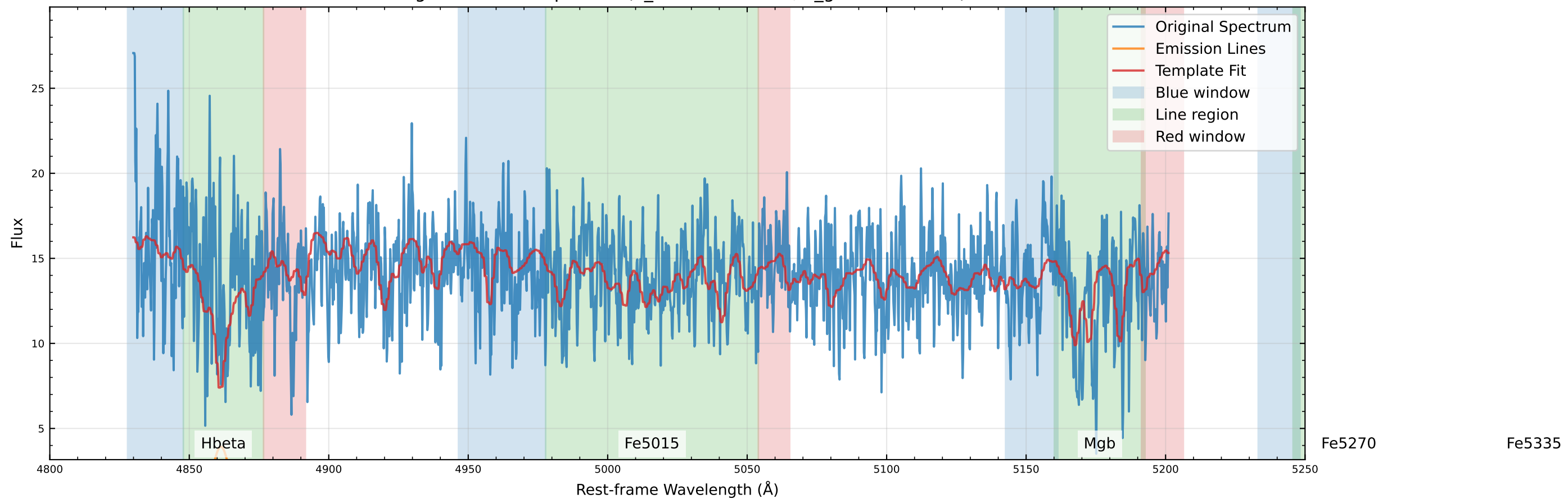
Original Data Comparison (v_star=78.0 km/s, v_gas=11.9 km/s)
