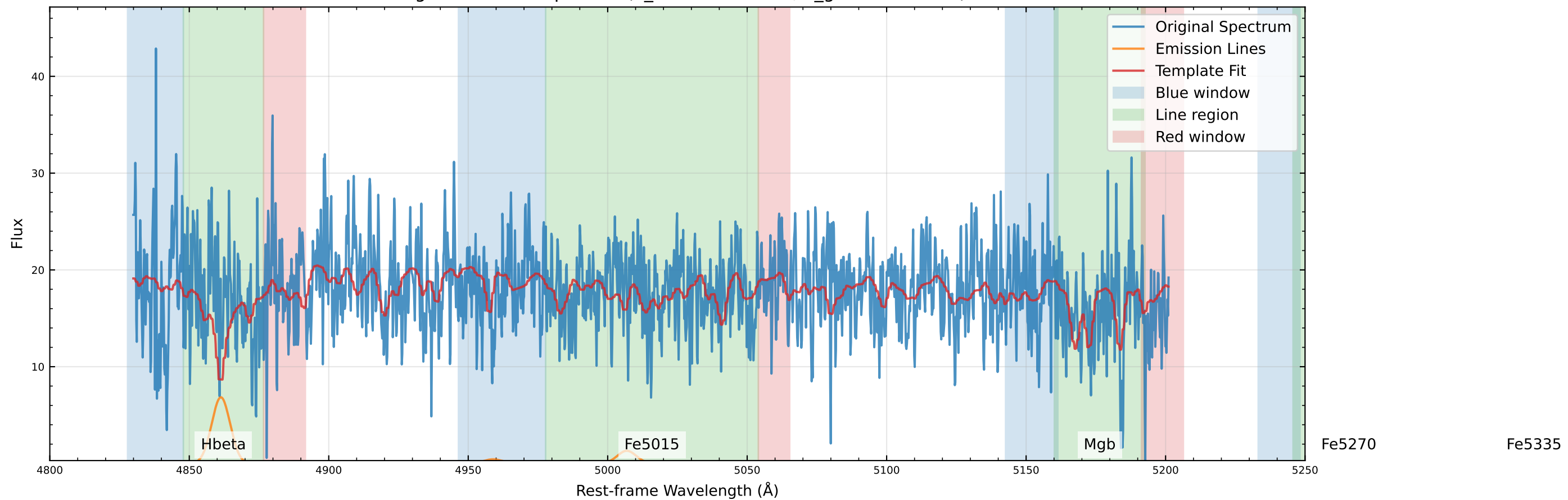
Original Data Comparison (v_star=42.1 km/s, v_gas=17.7 km/s)
