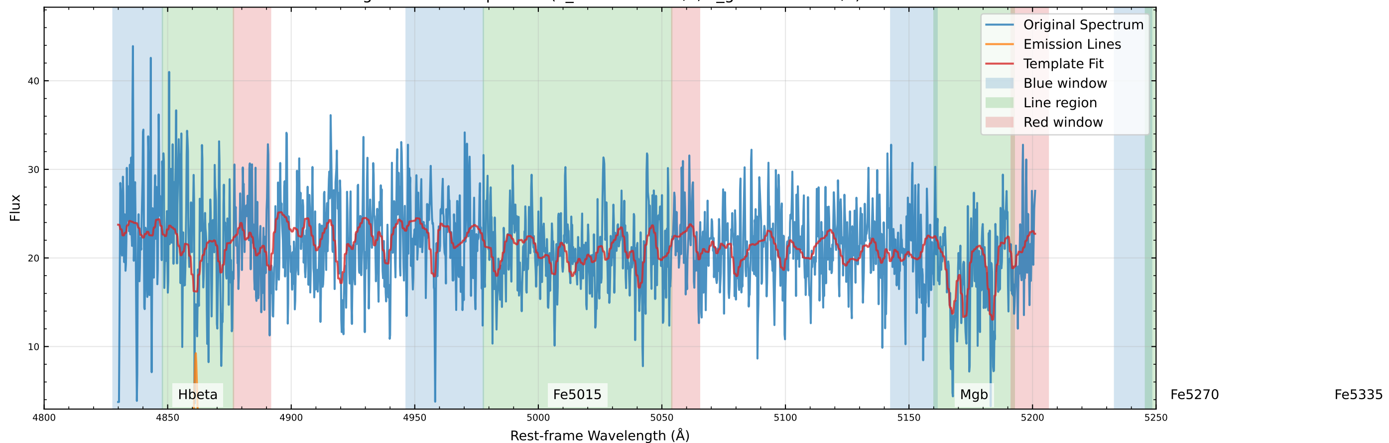
Original Data Comparison ( v_{\text{star}}=46.5 km/s, v_{\text{gas}}=135.3 km/s)
