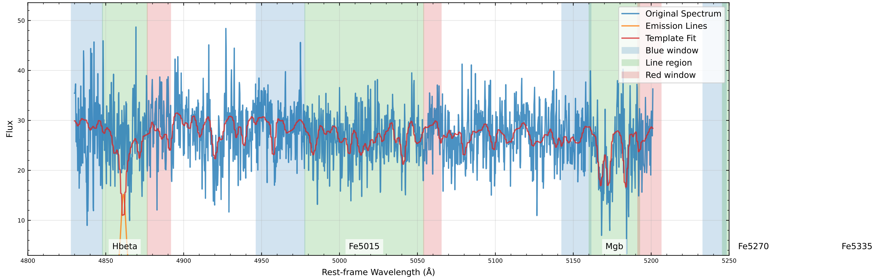
Original Data Comparison (v_star=44.7 km/s, v_gas=36.4 km/s)
