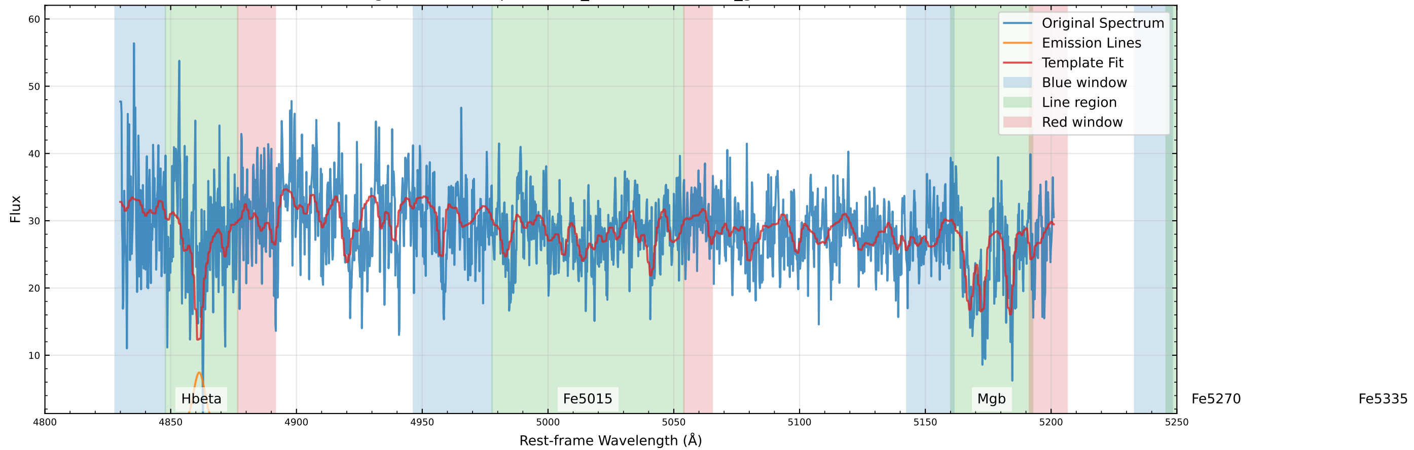
Original Data Comparison (v_star=62.9 km/s, v_gas=30.1 km/s)
